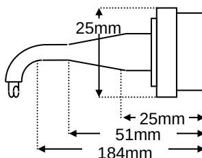
Cable Option 5 - End exit integral MI (mineral insulated) stainless steel cable
