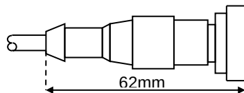
Cable Option 1 - End exit solder pins for customer to fit their own cable
