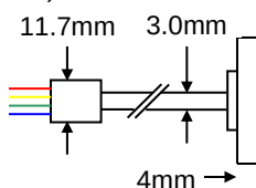
Cable Option 5 - End exit integral MI (mineral insulated) stainless steel cable
